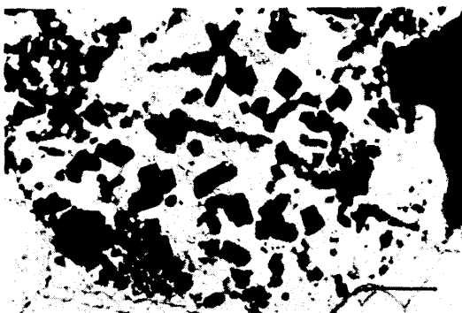
Fig. 7. Idiomorphic crystals of chromite enclosed in plagioclase. (a) Plane polarized light. (b) Reflected light. Scale bar is 0.05 mm in length.
